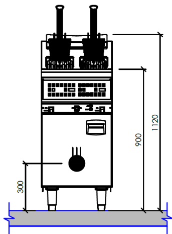
VISTA FRONTAL
